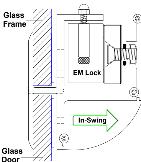
DSU Cover Bracket For Glass Frame & Glass Door
