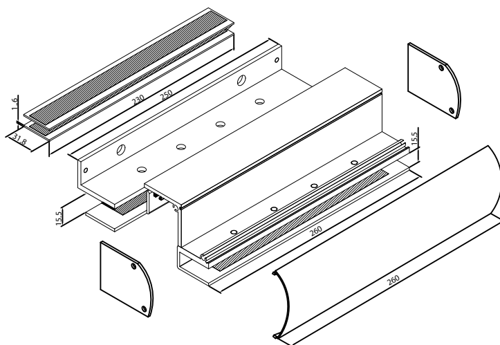
600C-DSU Cover Bracket Installation
