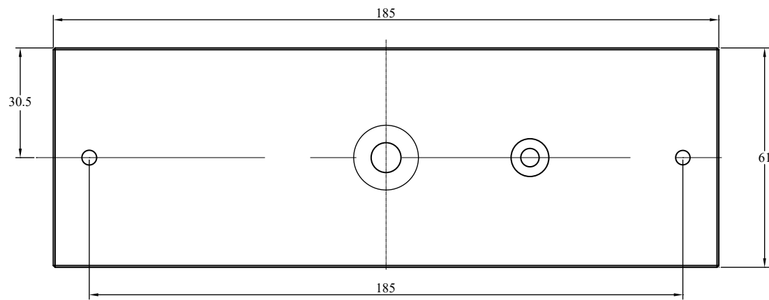
Armature Plate Dimension
