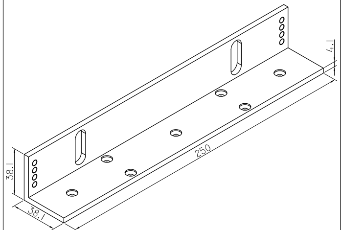
Specifications ( Unit = mm )
